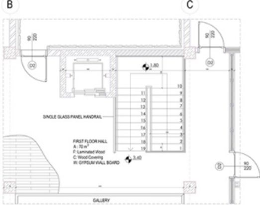
PARTIAL PLAN SCALE 1/20
