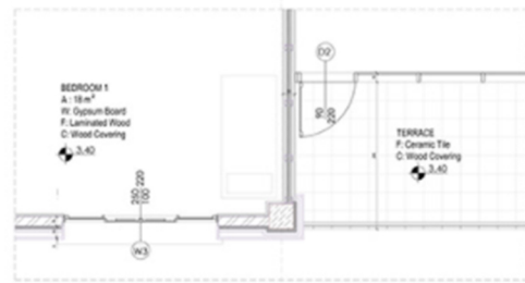
PARTIAL PLAN SCALE 1/20
