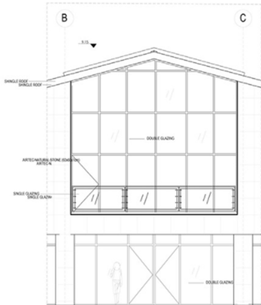
PARTIAL SECTION SCALE 1/20
